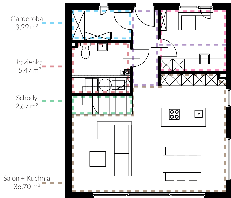
Parter: 65,43 m 2
